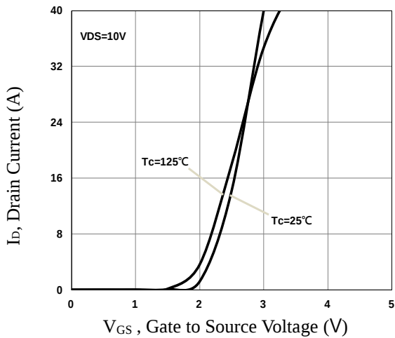
Fig.9 Transfer Characteristics
